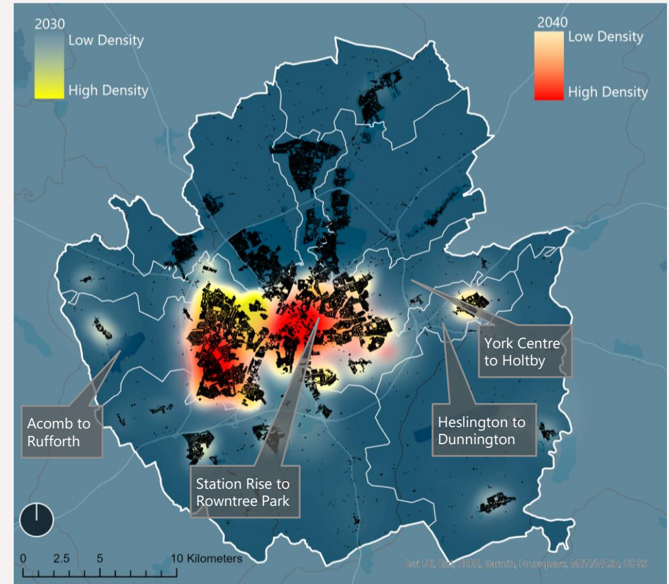
Density of buildings recommended for connection to district heat network in medium ambition scenario (red) and high (yellow)
